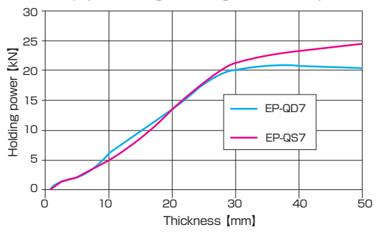
Holding power - thickness characteristic (4-pole holding, SS400 ground surface)
